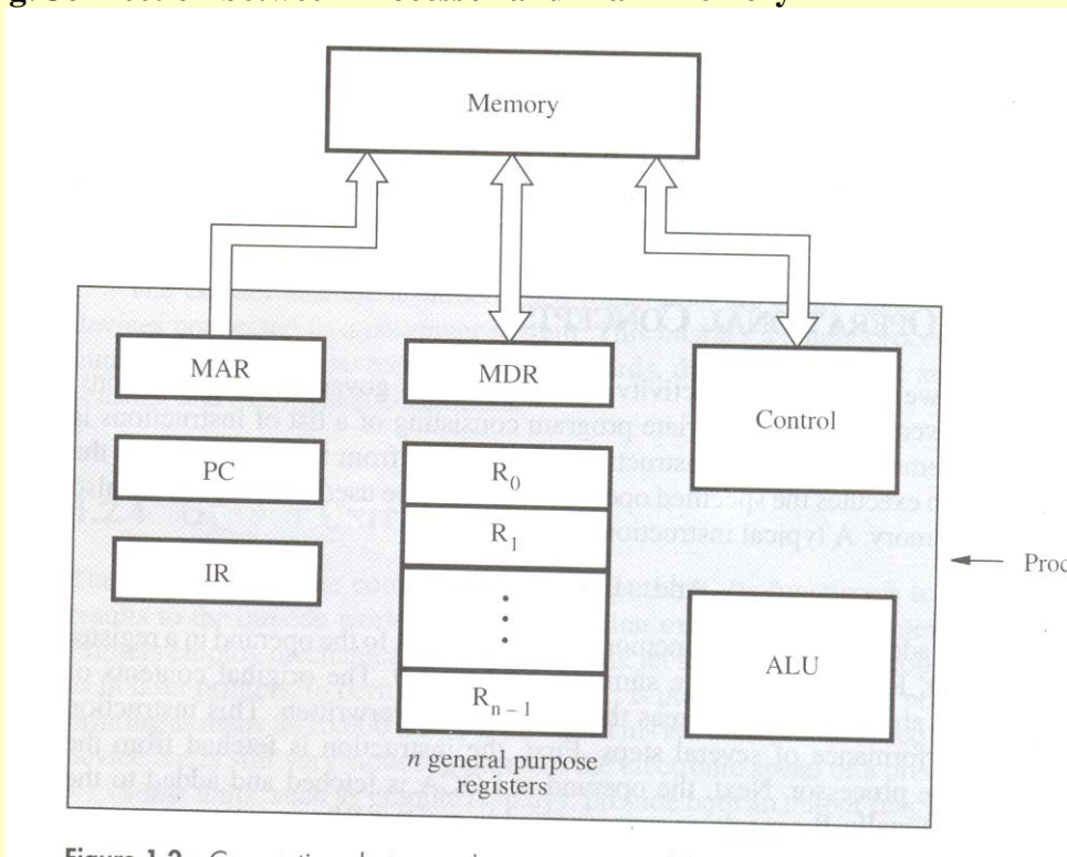
Figure 1.2 Connection between the processor and main memory
