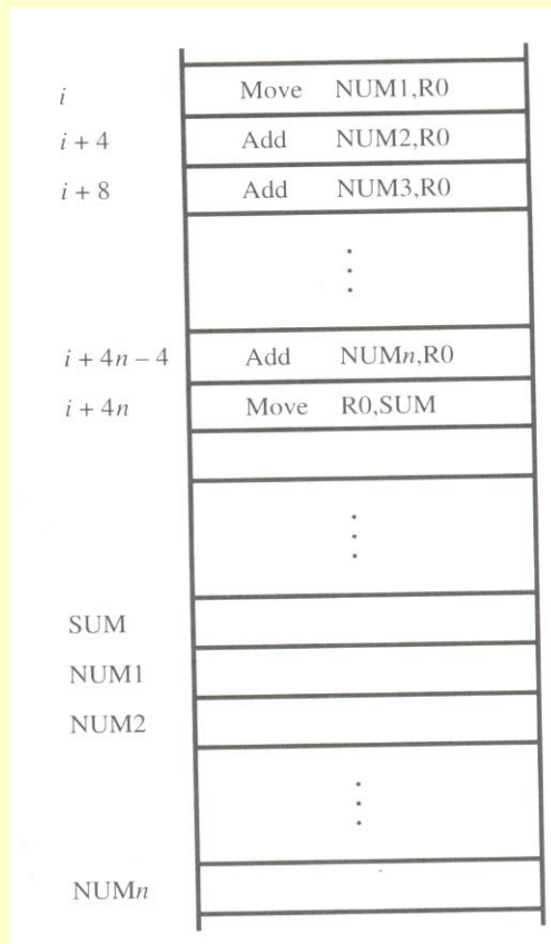
Fig: Straight Line Sequencing Program for adding 'n' numbers
